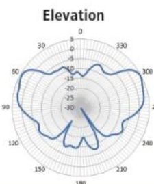
1950 MHz
