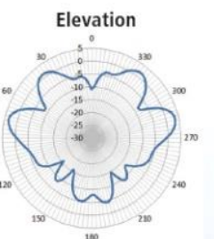
2700 MHz
